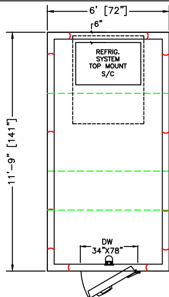
PLAN VIEW RIGHT HINGE
