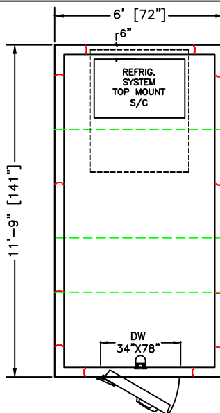
PLAN VIEW LEFT HINGE
