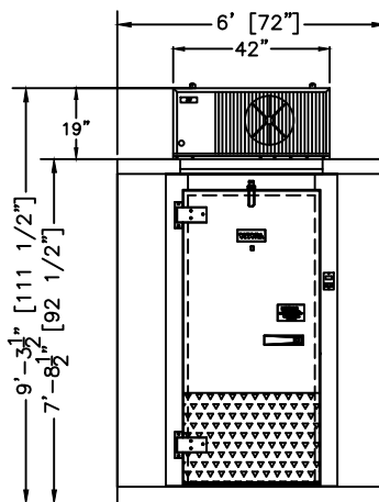
ELEVATION LEFT HINGE
